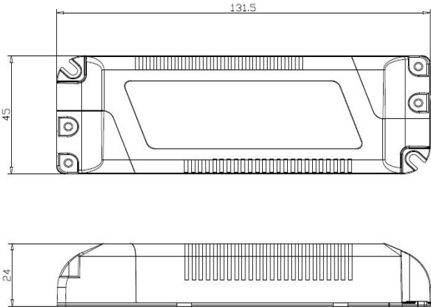
Unit: mm
